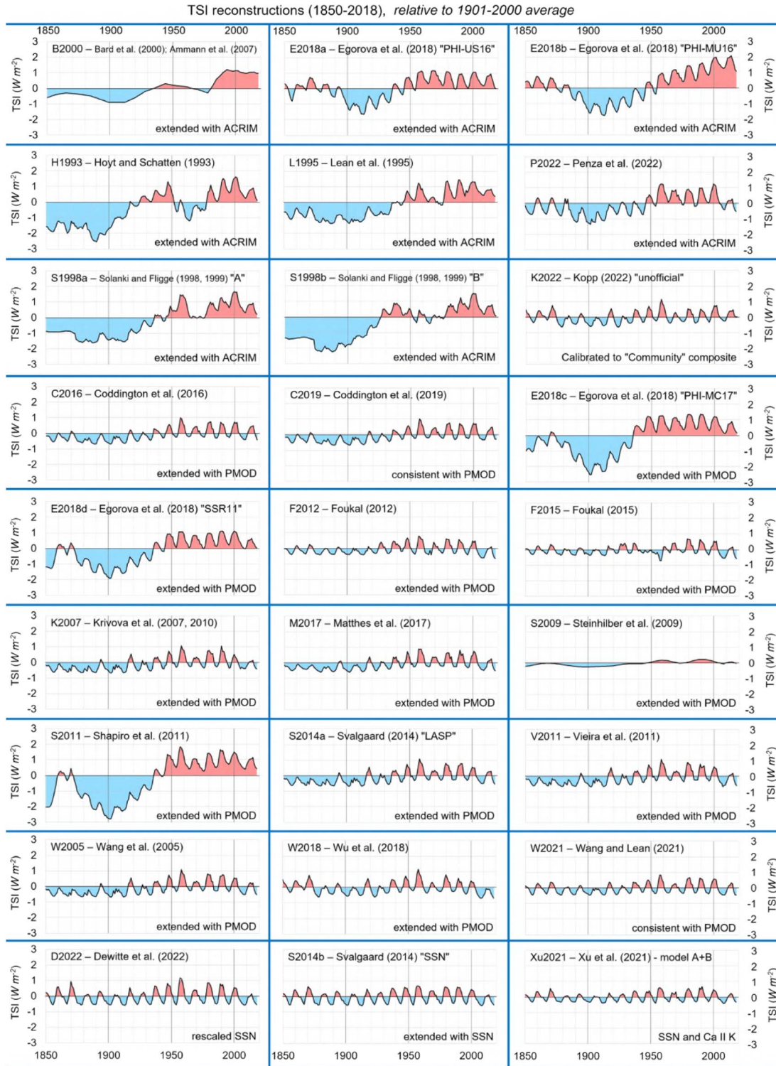
Figure 3. All 27 TSI estimates for the period 1850–2018, extended up to 2018 using either ACRIM or PMOD or SSN depending on the reconstruction. All estimates are plotted in units of W m^{-2} relative to their 20th century average. All estimates are denoted by the 1st letter and year of the original study—followed by a lower case letter if multiple estimates are available. The first eight panels are extended using ACRIM and listed alphabetically. K2022 was developed with the “Community” satellite composite (de Wit et al. 2017). The next 15 panels were extended or consistent with PMOD and are listed alphabetically. The final three panels are TSI estimates derived by scaling the SSN record, although Xu2021 also incorporate a rescaled Ca II K component.
