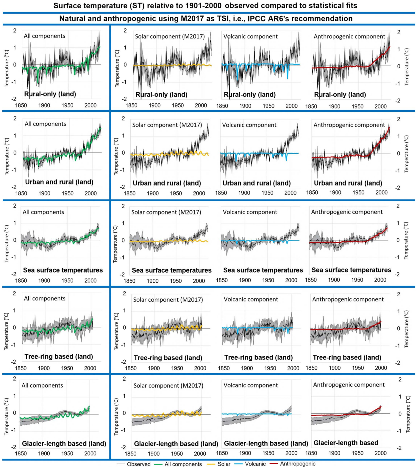
Figure 7. Breakdown of the natural and anthropogenic statistical fits for each of the ST estimates (thin black line for mean estimates; gray envelope for associated uncertainty bands) using IPCC AR6's recommended M2017 TSI series. The left-hand panels correspond to the best fits using all components (thick green line). The other panels correspond to—from left to right: the solar component (thick yellow line); volcanic component (thick blue line); anthropogenic component (thick red line). Each row corresponds to a different ST record—from top to bottom: rural-only; urban and rural; SSTs; tree-ring based; glacier-length based.
