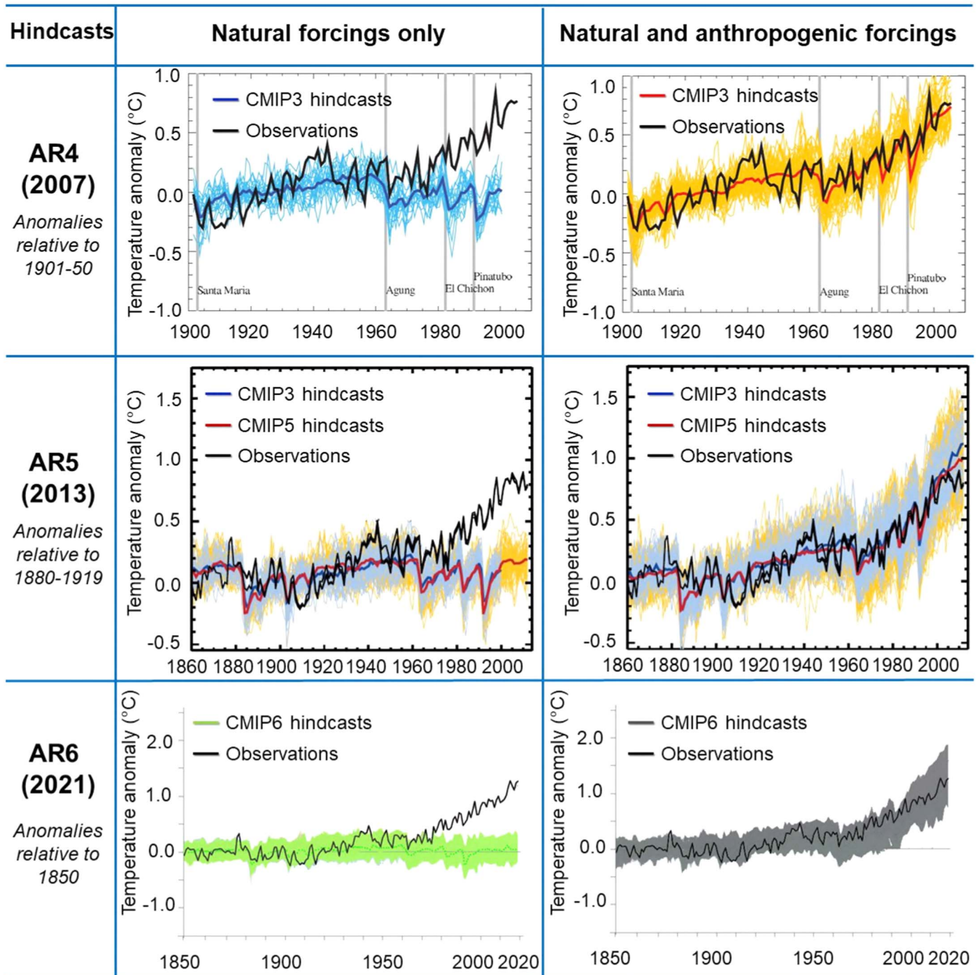
Figure 1. Summary of the detection and attribution hindcasting experiments presented by the IPCC in (top) AR4; (middle) AR5; (bottom) AR6. Left-hand panels compare the hindcasts using “natural forcings only” to the average global ST records (thick black lines labeled “Observations”) considered by each report. Right-hand panels present the equivalent analysis using the hindcasts with both “natural and anthropogenic forcings.” For AR4 and AR5, each thin colored line corresponds to a separate hindcast and the thick colored lines represent the multi-model mean hindcast. For AR6, the shaded envelope represents the 5%–95% range of individual simulations and the dotted lines represent the multi-model mean hindcast. AR4 panels are adapted from Figure 9.5 of IPCC (2007). AR5 panels are adapted from Figure 10.1 of IPCC (2014). AR6 panels are adapted from Figure FAQ 3.1 of IPCC (2021).
