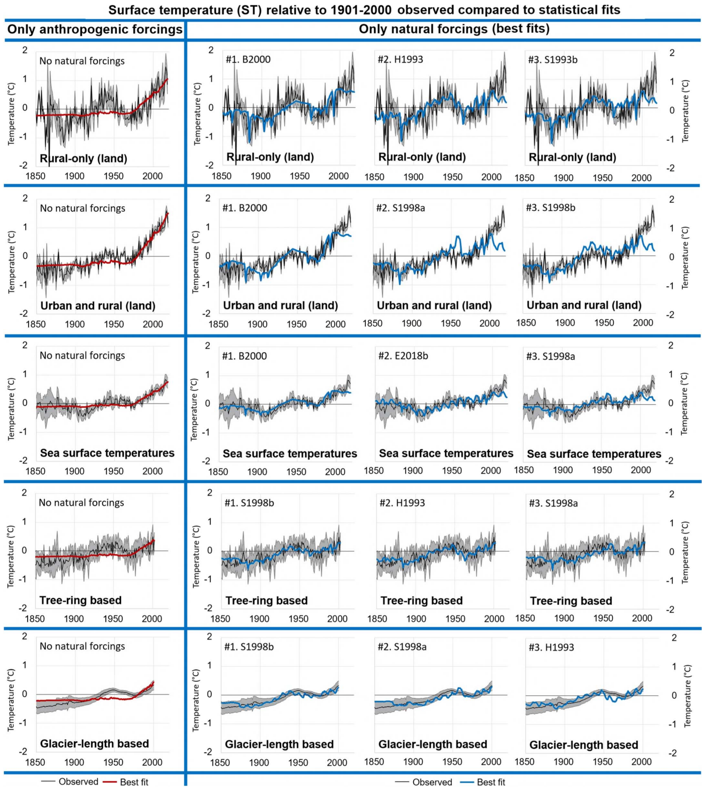
Figure 6. Comparison of the various ST estimates (thin black line for mean estimates; gray envelope for associated uncertainty bands) to some of the statistical fittings. The left-hand panels correspond to the best fits using only anthropogenic forcings (thick red line). The other panels correspond to the three best statistical fits (in terms of r^2 ) using only natural forcings (thick blue line). Each row corresponds to a different ST record—from top to bottom: rural-only; urban and rural; SSTs; tree-ring based; glacier-length based.
