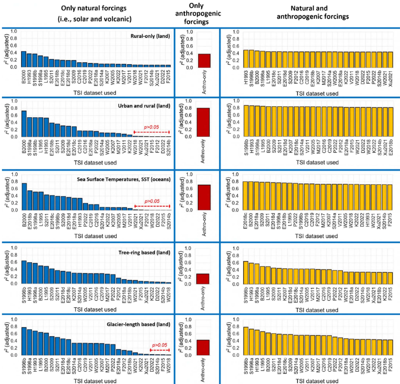
Figure 4. Adjusted r^2 statistics for all multilinear regression fittings. The higher the r^2 value (from 0 to 1), the more of the observed temperature series could be explained in terms of the components used in the statistical fitting. Left-hand panels correspond to the fittings using only natural forcings (solar and volcanic) with the results for each TSI data set ranked from best fit (left) to worst fit (right). All fits were statistically significant ( p < 0.05 ), except for the weakest fits highlighted with the p > 0.05 label. Middle panels show the results using only the anthropogenic forcings series. Right-hand panels correspond to the combined “natural and anthropogenic” fits. Each row corresponds to a different ST record—from top to bottom: rural-only; urban and rural; SSTs; tree-ring based; glacier-length based.
