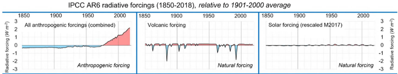
Figure 2. The (left) anthropogenic, (middle) volcanic and (right) solar components recommended by IPCC AR6 for GCM hindcasts—taken from IPCC AR6 WG1 Annex III data set (IPCC 2021) that we downloaded from https://doi.org/10.5281/zenodo.5705391 . All three components are plotted for the period 1850–2018 in terms of “radiative forcing” in units of \text{W m}^{-2} relative to their 20th century average.
