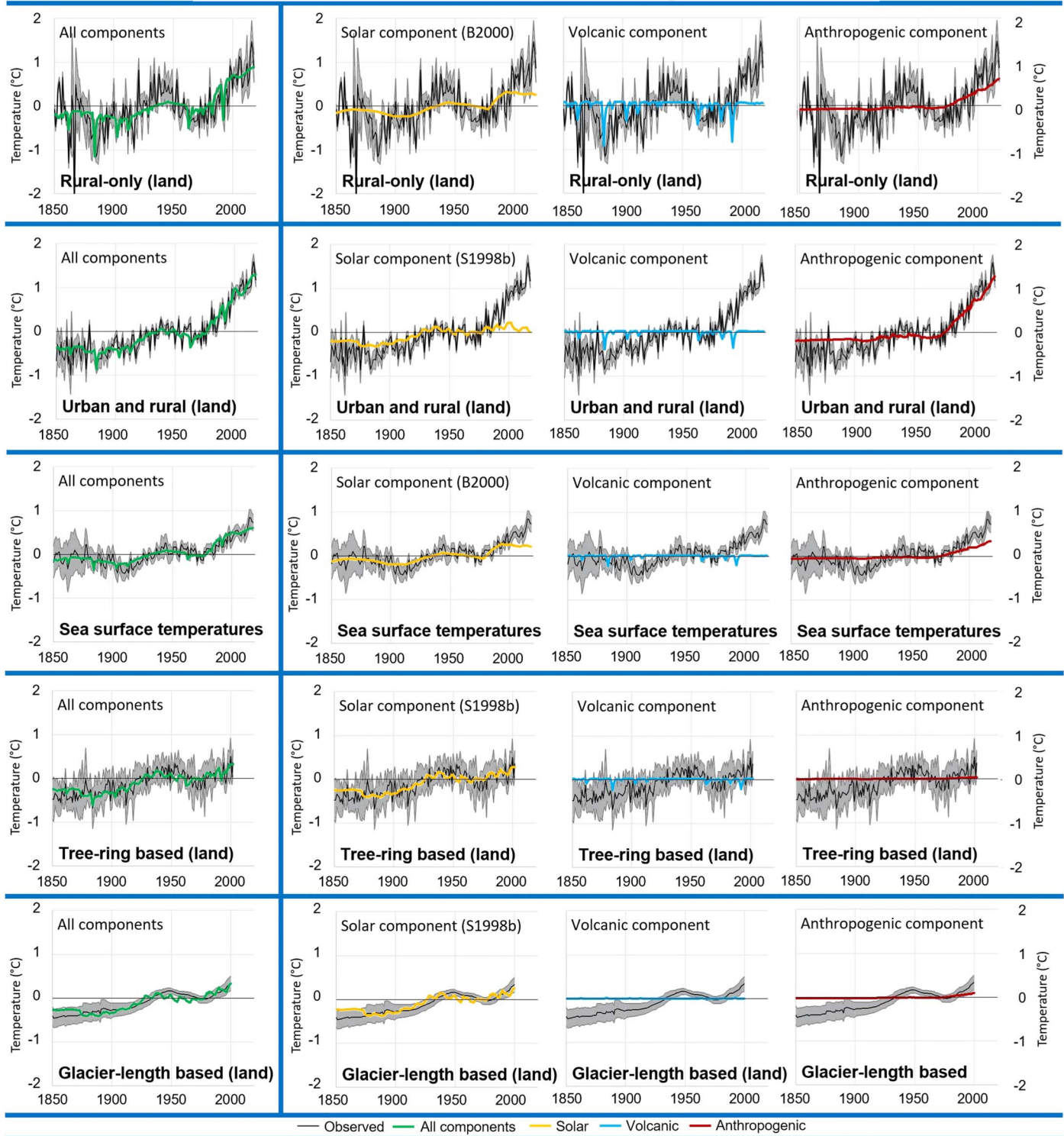
Figure 8. Breakdown of the natural and anthropogenic statistical fits for each of the ST estimates (thin black line for mean estimates; gray envelope for associated uncertainty bands) using the TSI series that maximizes the solar contribution to the long-term warming. The left-hand panels correspond to the best fits using all components (thick green line). The other panels correspond to—from left to right: the solar component (thick yellow line); volcanic component (thick blue line); anthropogenic component (thick red line). Each row corresponds to a different ST record—from top to bottom: rural-only; urban and rural; SSTs; tree-ring based; glacier-length based.
