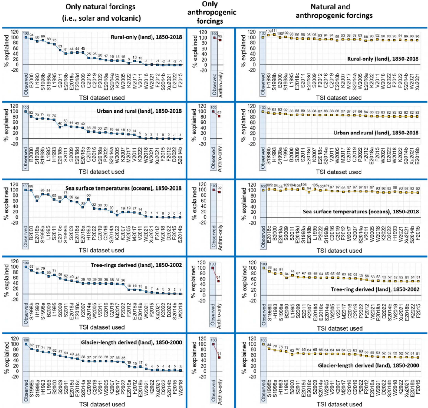
Figure 5. Percentages of the long-term warming linear trend for all multilinear regression fittings to each of the temperature series. The linear trends were calculated over the maximum overlap period: 1850–2018 for the three instrumental estimates; 1850–2002 for the tree-ring based proxies; 1850–2000 for the glacier-length based proxies. As for Figure 4, left-hand panels correspond to the fittings using only natural forcings (solar and volcanic) with the results for each TSI data set ranked as in Figure 4, i.e., from best fit (left) to worst fit (right). Middle panels show the results using only the anthropogenic forcings series. Right-hand panels correspond to the combined “natural and anthropogenic” fits. Each row corresponds to a different ST record—from top to bottom: rural-only; urban and rural; SSTs; tree-ring based; glacier-length based.
