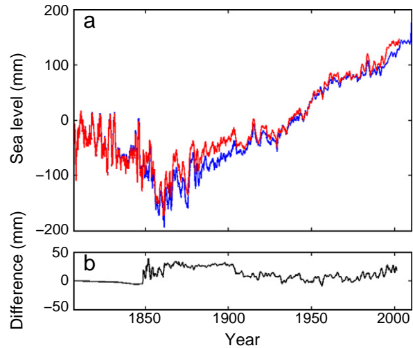
Fig. 6. Panel (a): GSL06 (red) and present study GSL12 (blue); panel (b) is the difference between two reconstruction (GSL06–GSL12). (For interpretation of the references to colour in this figure legend, the reader is referred to the web version of this article.)
